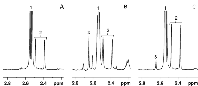
Figure 2. 1 H-NMR spectra (600 MHz) for 2 mM methionine (H 2 O/D 2 O 9:1 (v/v), pH 3.0 ± 0.1) exposed to light in the NMR tube in the presence of 0.2 mM riboflavin and 2 mM gallic acid (three fluorescent lamps) in an air condition. (A) control sample (dark condition); (B) after 15 min of light exposure; (C) after 15 min of light exposure with 2 mM gallic acid. Assignments are as follows: 1, methionine γ-CH 2 ; 2, riboflavin 6-CH 3 (low field) and 7-CH 3 (high field); 3, methionine sulfoxide S(O)CH 3 .
